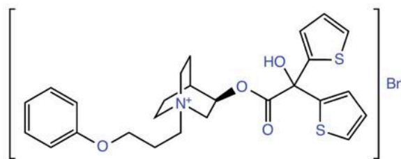
Acridinium bromide
