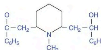
Lobeline
