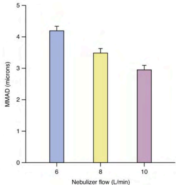
• Fig. 3.15 Effect of power gas flow rate on the mass median aerodynamic diameter (MMAD) of aerosol particles produced on average by 17 gas-powered nebulizers. (From Hess, D., Fisher, D., Williams, P., et al. [1996]. Medication nebulizer performance: effects of diluent volume, nebulizer flow, and nebulizer band. Chest , 110, 498.)
